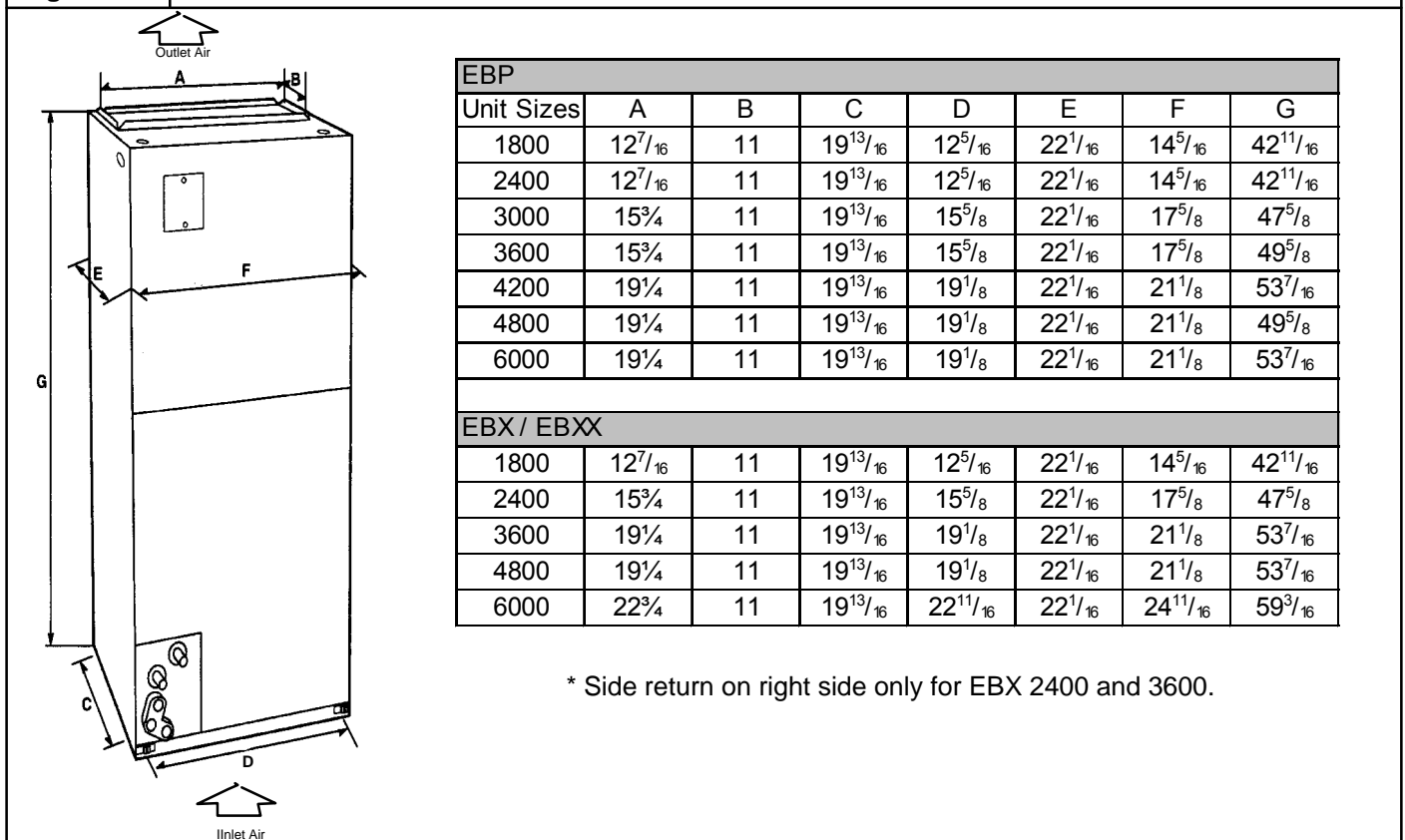
Figure 1 Unit Dimensions
